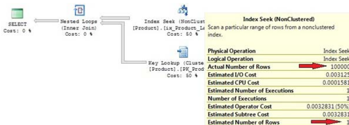
Picture 5: Execution plan created by use of stale statistics
